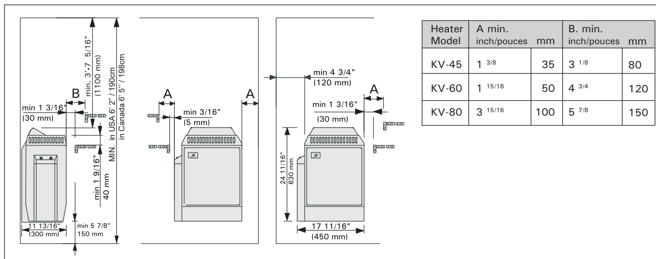
Figure 5. Min. distances to combustible materials
